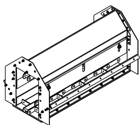
Extension section with side inlet for pit
