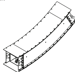
1 m extension section for SR40 as 30° bend. Also available as 15° (0.5 m) and 45° (1.5 m)
