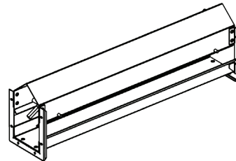
Extension section with side inlet for pit incl. chain
